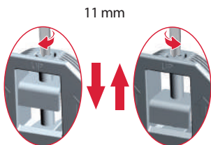
VERTICAL ADJUSTMENT
