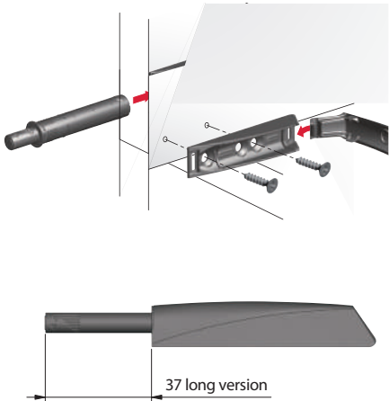
INSTALLATION THROUGH ADAPTER HOUSING
