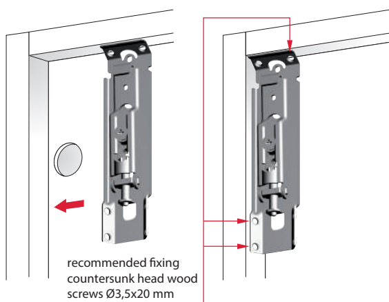
ADJUSTMENTS
