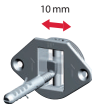
LATERAL ADJUSTMENT
