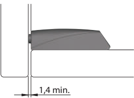
WITH BUFFER for cabinets using sprung hinges.
