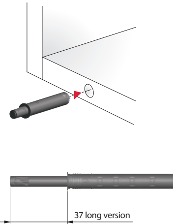
INSTALLATION TO BE EMBEDDED INSIDE THE PANEL
